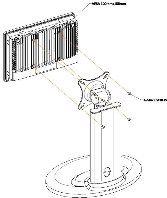
Figure 10 EX-91910CP VESA Mounting
