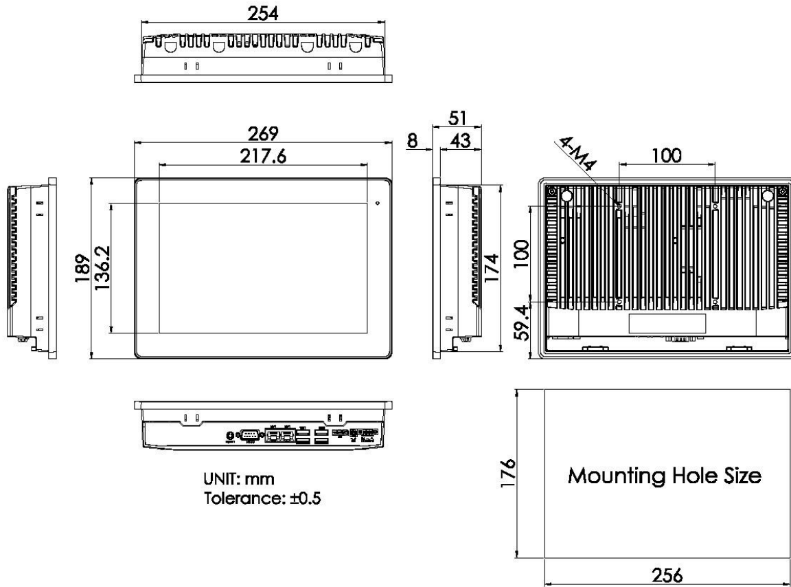
Figure 1 Dimensions of EX-91910CP
