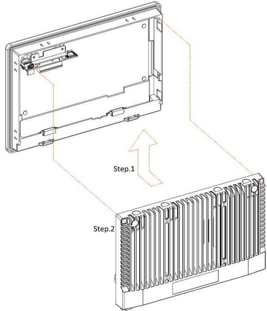
Figure 15 EX-91910CP MB Box kit attaches to Front Kit
