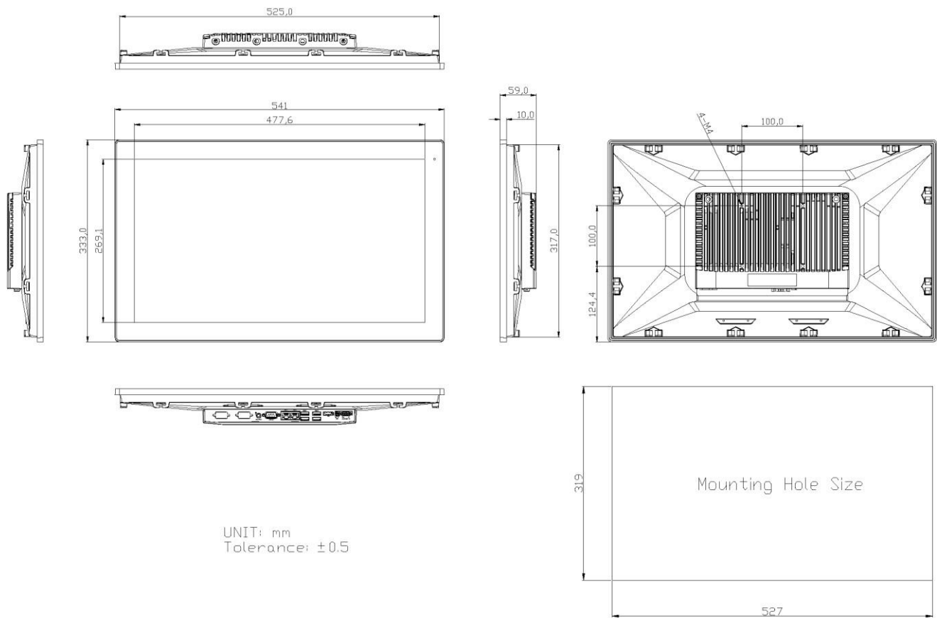
Figure 3 Dimensions of EX-91921CP
