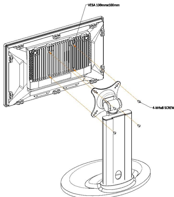
Figure 11 EX-91916CP/EX-91921CP VESA Mounting
