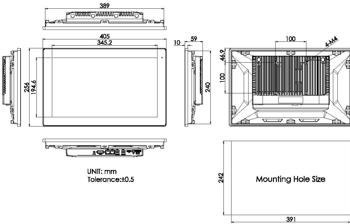
Figure 1 Dimensions of EX-91910CP
