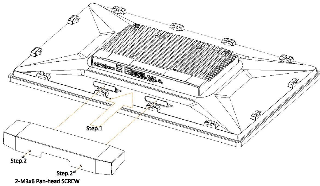
Figure 14 EX-91916CP/EX-91921CP Cable Cover Installation
