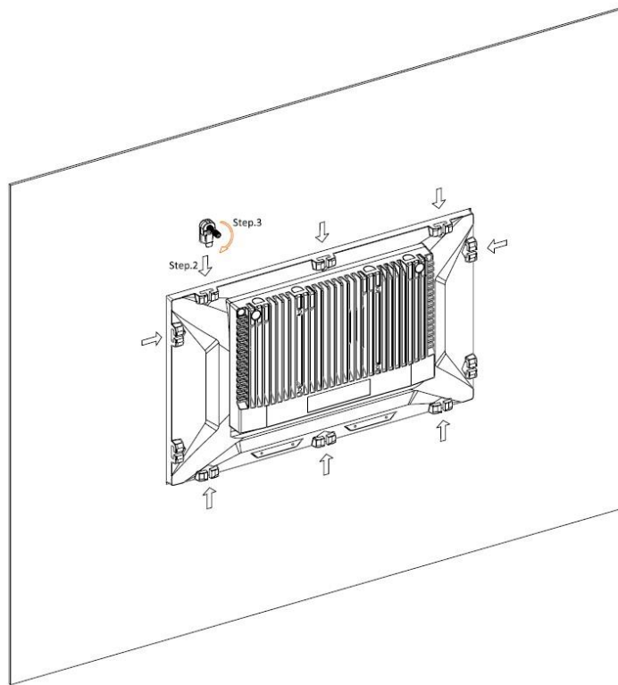
Figure 13 EX-91916CP/EX-91921CP Panel Mounting
