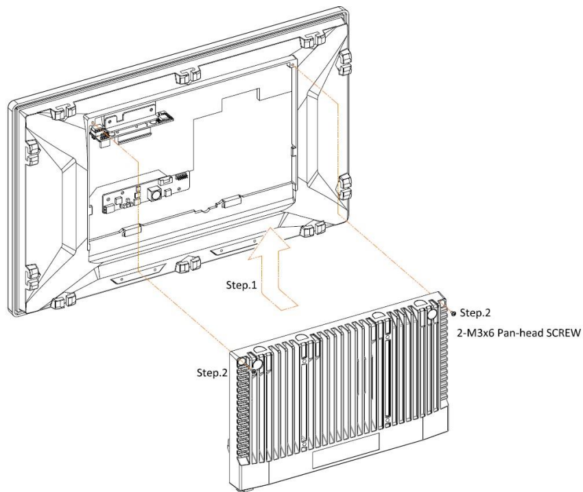
Figure 16 EX-91916CP/921CP MB Box kit attaches to Front Kit
